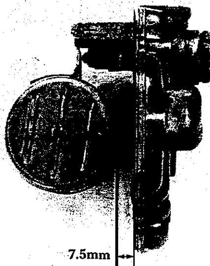
Weber floats being set to 7.5mm with the needle and seat just touching.
