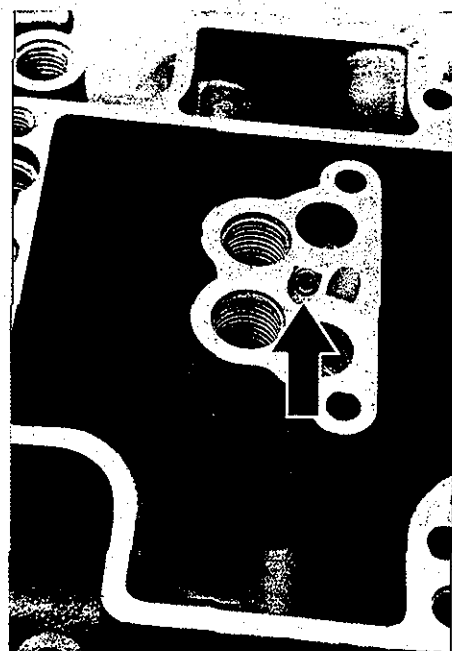
Dellorto emission control carburettor has high mounted air bleeds to the idle jets. Take the cover off to check the position. Look for the brass sleeves clearly visible in the two small recesses as arrowed.
