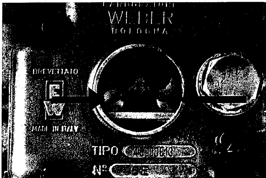
Weber carburettor with cover removed showing the position of the idle jets.
