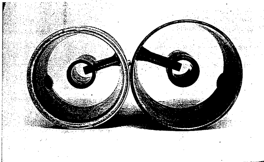
Dellorto 40mm 7848.1 auxiliary venturi on the left, and 45mm - 48mm 8011.1 auxiliary venturi on the right.
