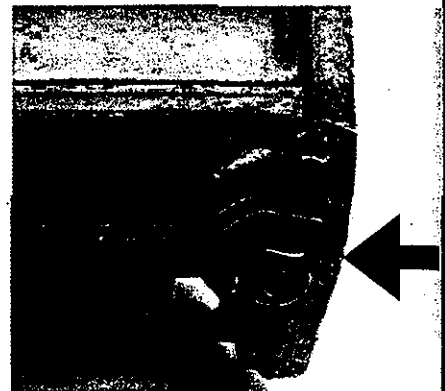
Dellorto with plain throttle spindle cover (arrowed) correctly fitted. Note how tab of lockwasher is turned up to lock the nut.
